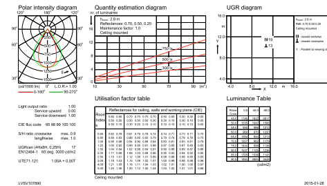
IFGU_4MX400 G3 491 1xLED55S/840 PSD NB-General uniform lighting
