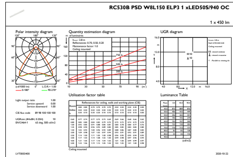
IFGU1_RC530BPSDW8L150ELP31xLED50S940OC
