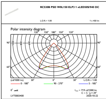
OFPC1_RC530BPSDW8L150ELP31xLED50S940OC
