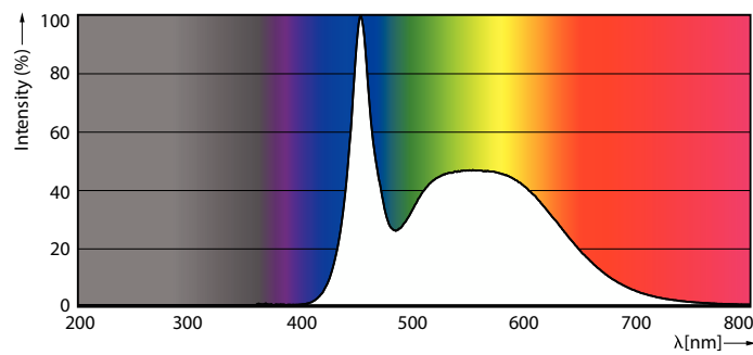
Spectral Power Distribution Colour - TForce Core HB MV ND 55W E40 865 G3
