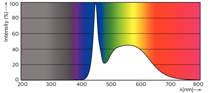
Spectral Power Distribution Colour - LED PLC 8.5W 865 2P G24d-3
