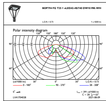
OFPC1_BDP794FGT251xLED42-4S740DW10MK-WH
