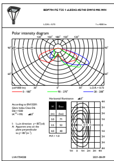
OFPL1_BDP794FGT251xLED42-4S740DW10MK-WH
