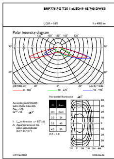
OFPL1_BRP776FGT251xLED49-4S740DW50
