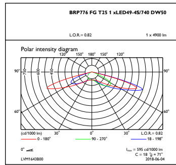
OFPC1_BRP776FGT251xLED49-4S740DW50
