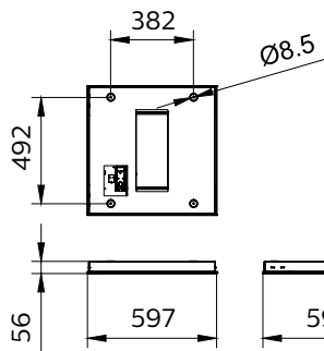
SM100C LED37S 865 W603L603 PSU UNV G3
