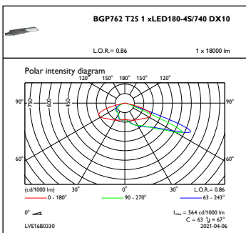
OFPC1_BGP762T251xLED180-4S740DX10
