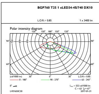
OFPC1_BGP760T251xLED34-4S740DX10
