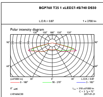
OFPC1_BGP760T251xLED27-4S740DS50
