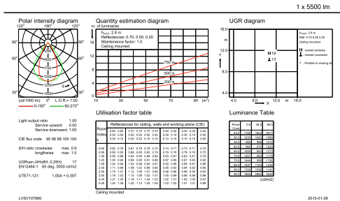
IFGU_4MX400 G3 491 1xLED55S/840 PSD NB-General uniform lighting
