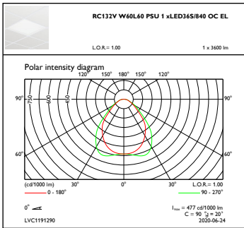
OFPC1_RC132VW60L60PSU1xLED36S840OCEL
