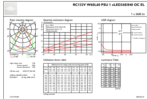
IFGU1_RC132VW60L60PSU1xLED36S840OCEL
