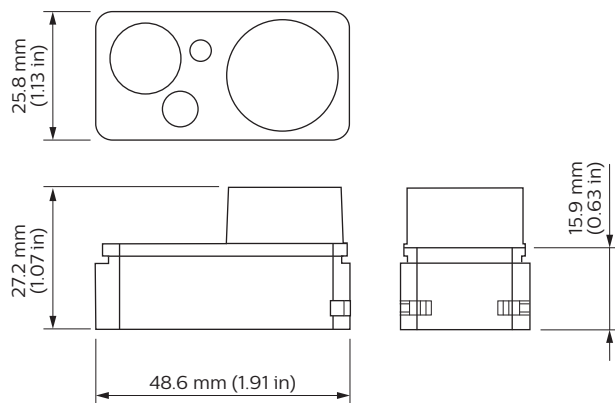
LRI1667 sensor dimensions in mm.
