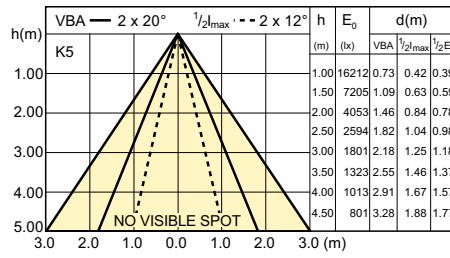
LDBE_CDMR111E_0008-Beam diagram
