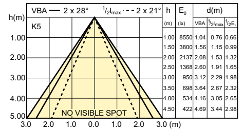
LDBE_CDMR111E_0009-Beam diagram
