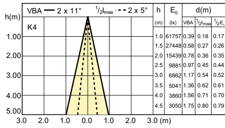
LDBE_CDMR111E_0007-Beam diagram
