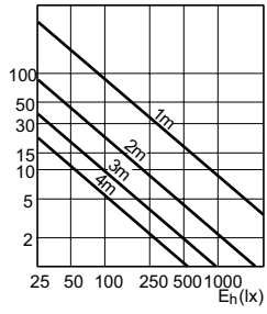
LDAC_CDM-R111_35W_24D-Accent diagram
